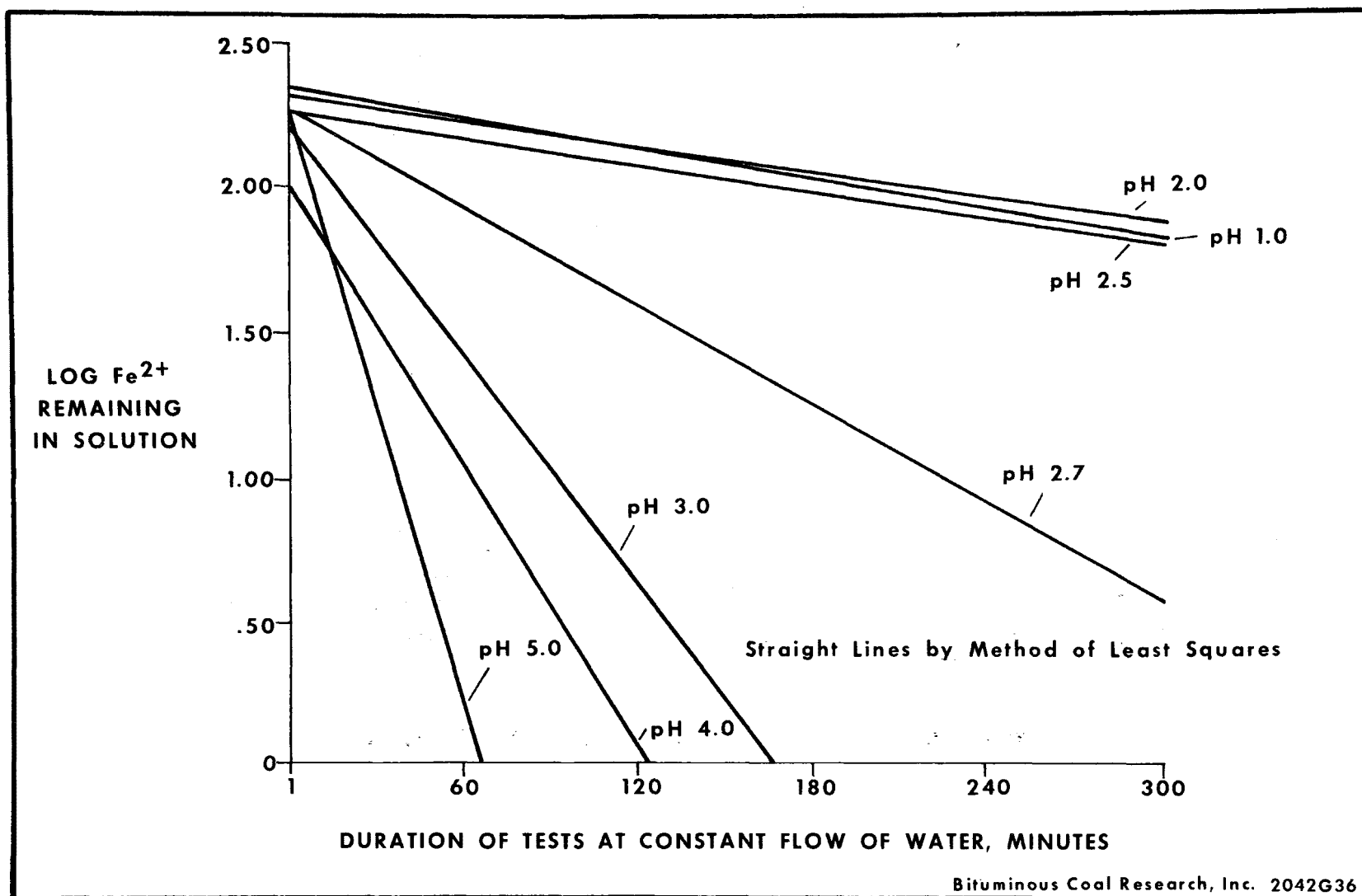
Figure 4. Effect of pH on Rate of Adsorption of Fe 2+ on Activated Carbon
